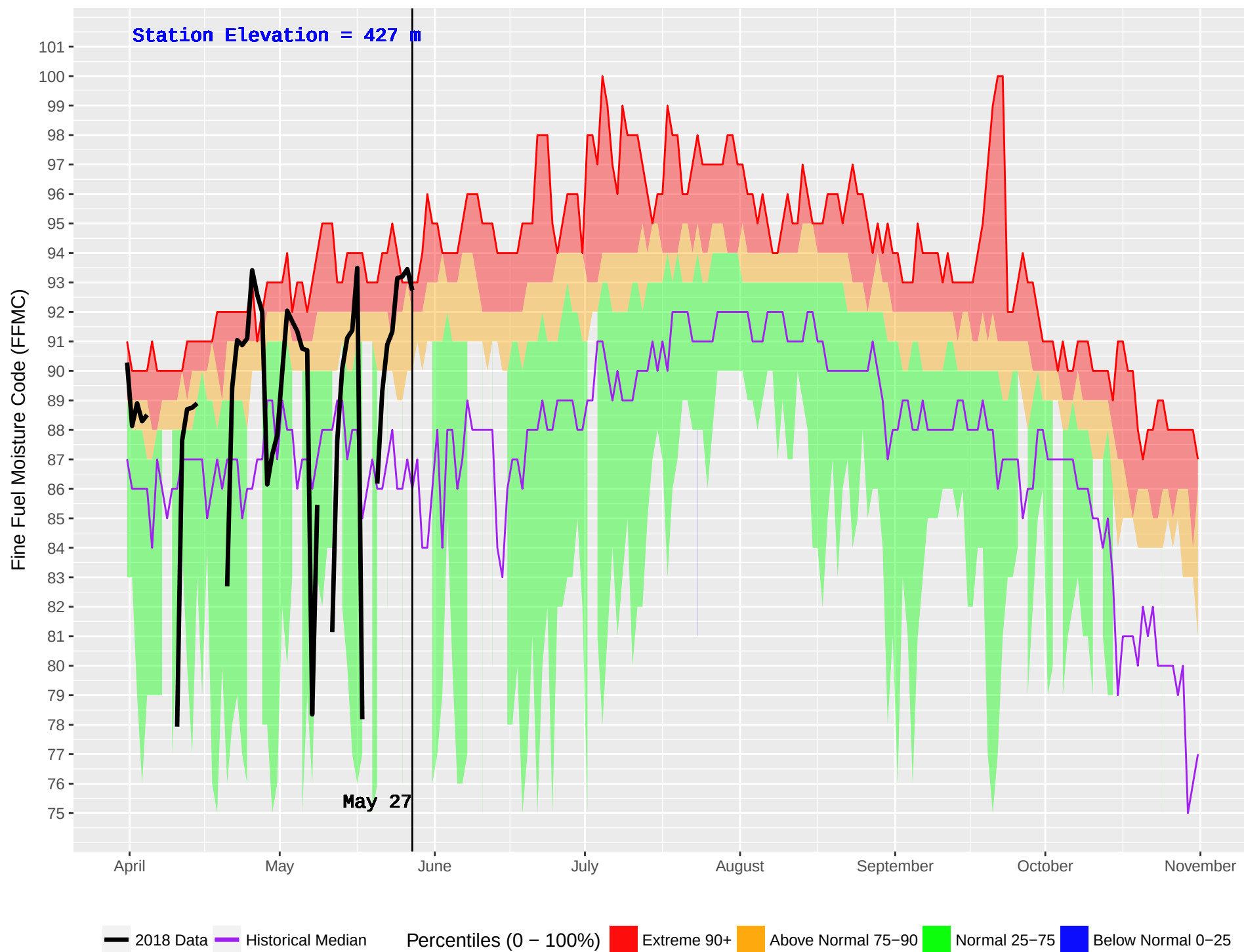
PENTICTON RS (328) : Historical (1970–2016) and Current (2018) Noon Fine Fuel Moisture Code (FFMC)
